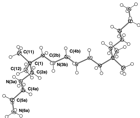
Fig. 6 Projection of the centrosymmetric [H_6L^6]^{6+} cation in compound 5 . A figure showing the unit cell contents of [H_6L^6]Cl_6 \cdot 2H_2O , 5 , down a , and indicating short hydrogen-bonded contacts is deposited as ESI.
