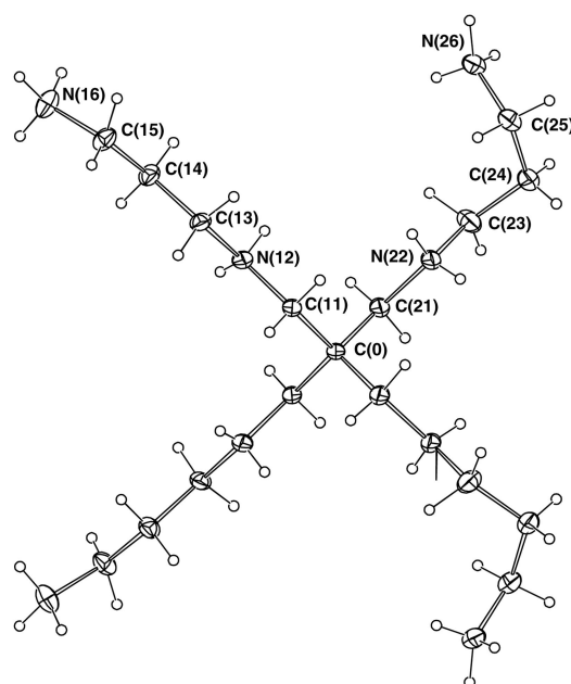
Fig. 3 The [\text{H}_8\text{L}^8]^{8+} cation, in the octachloride salt, 8 , projected normal to the crystallographic 2 axis which lies horizontal in the page. A figure showing the unit cell contents, projected down c , is deposited as ESI.
