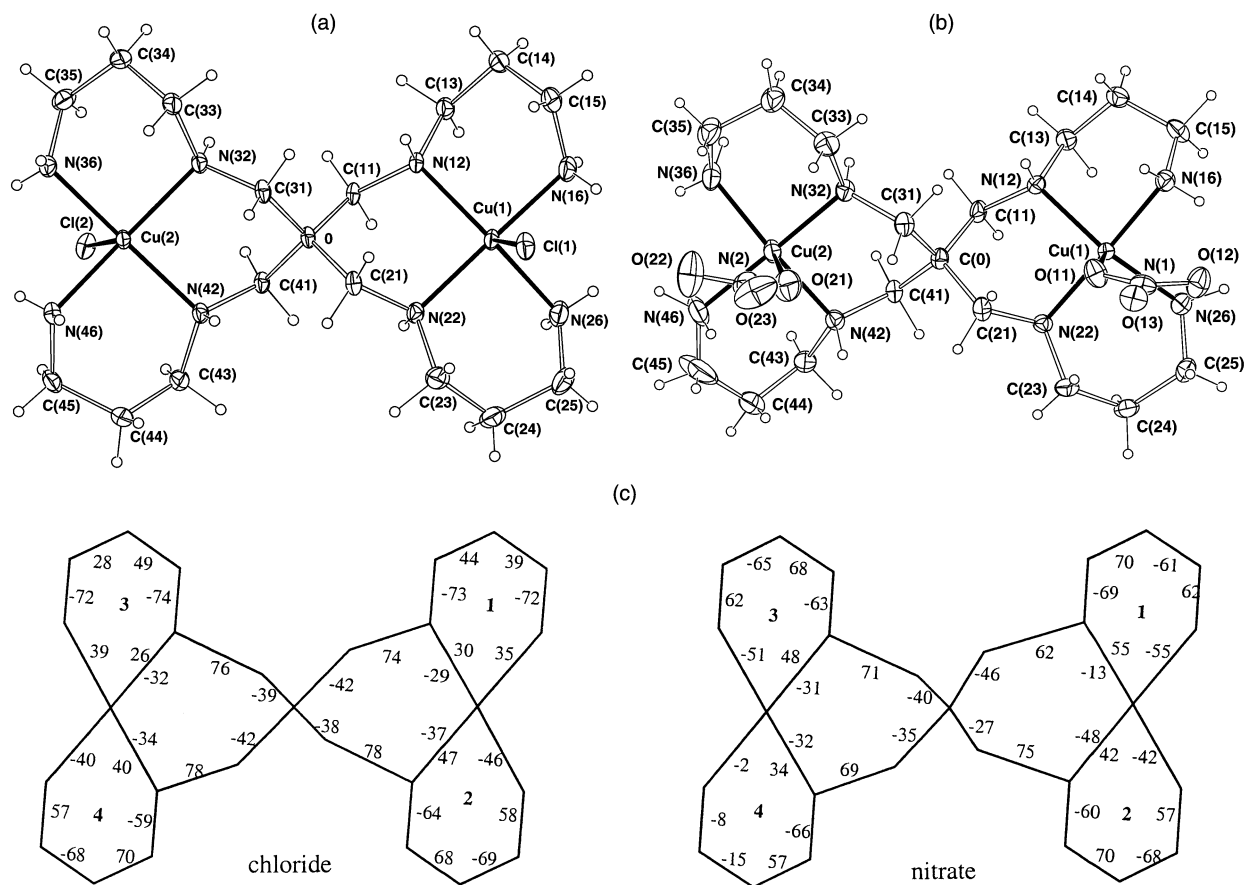
Fig. 4 Projections of the cations of [(\text{CuX})_2\text{L}^8]\text{X}_2 \cdot n\text{H}_2\text{O} (a) 9 , \text{X} = \text{Cl} , n = 2 , and (b) 10 , \text{X} = \text{NO}_3 , n = 3 normal to the moiety 'plane'. (c) Schematic diagram of the intra-ring torsion angles as descriptors of ring conformations for the two complexes (s.u.'s typically 0.3, 0.6°).
