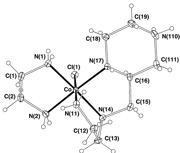
Fig. 8 Projection of the [\text{Co}(\text{HL}^5)(\text{en})\text{Cl}]^{3+} cation in complex 7.
