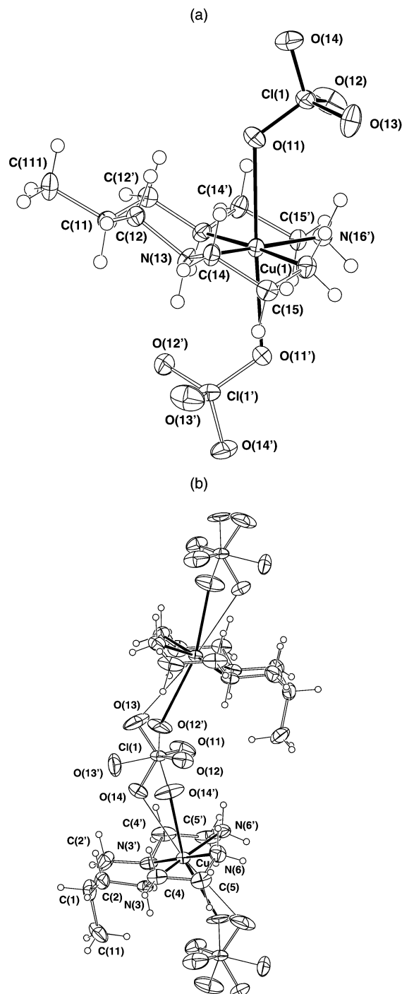
Fig. 7 (a) A single molecule (molecule 1) of [Cu(L^1)(OCIO_3)_2] , 2 (molecule 2 is similar). (b) Projection of the polymeric cation of [Cu(L^1)(OCIO_2O)]^+_{(x/2)} , 3 , showing the modelling of the perchlorate in terms of components rotationally disordered about Cl–O(1), entailing coordination via O(13,14) or O(12',14').
