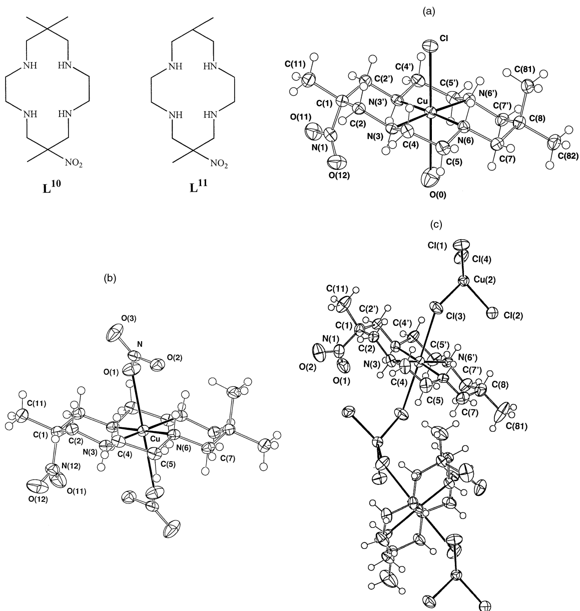
Fig. 10 Projections of: (a) The [\text{Cu}(\text{L}^{10})\text{Cl}(\text{OH}_2)]^+ cation of 12 ; (b) the centrosymmetric [\text{Cu}(\text{L}^{10})(\text{ONO}_2)]^+ cation of 13 (the nitro group is scrambled with its inversion-related methyl counterpart; one isolated complex unit is shown) and (c) the asymmetric unit of complex 14 in its one-dimensional polymeric stack. A figure of the unit cell contents of 12 , projected down a , showing the stacking of cations up that axis, is deposited as ESI.
