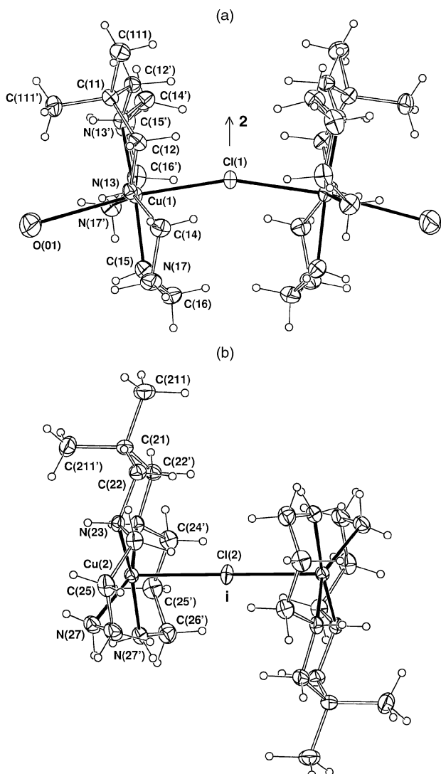
Fig. 2 (a),(b) Projections of the two cations of [\{\text{Cu}(\text{L}^3)(\text{OH}_2)_2\text{Cl}][\{\text{Cu}(\text{L}^3)_2\text{Cl}]\text{ClO}_4 , 6 , cation 1 lying on a crystallographic 2 axis, and 2 about an inversion centre. A figure showing the unit cell contents, projected down b , is deposited as Electronic Supplementary Material (ESI).
