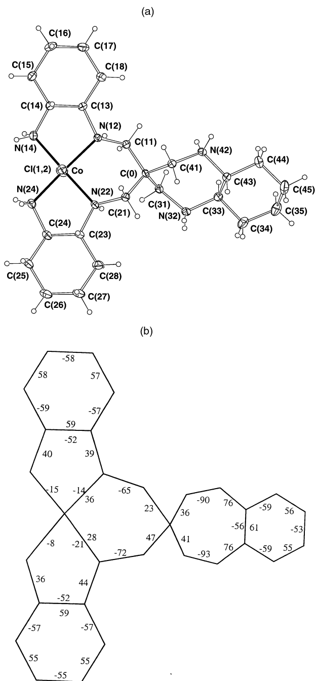
Fig. 9 (a) Projection of the \text{trans-[Co(H}_2\text{L}^9\text{)Cl}_2\text{]}^{3+} cation in 11 , down the Cl–Co–Cl line. (b) Torsion angles (to nearest degree) within the rings (s.u.'s are typically 0.5°).
