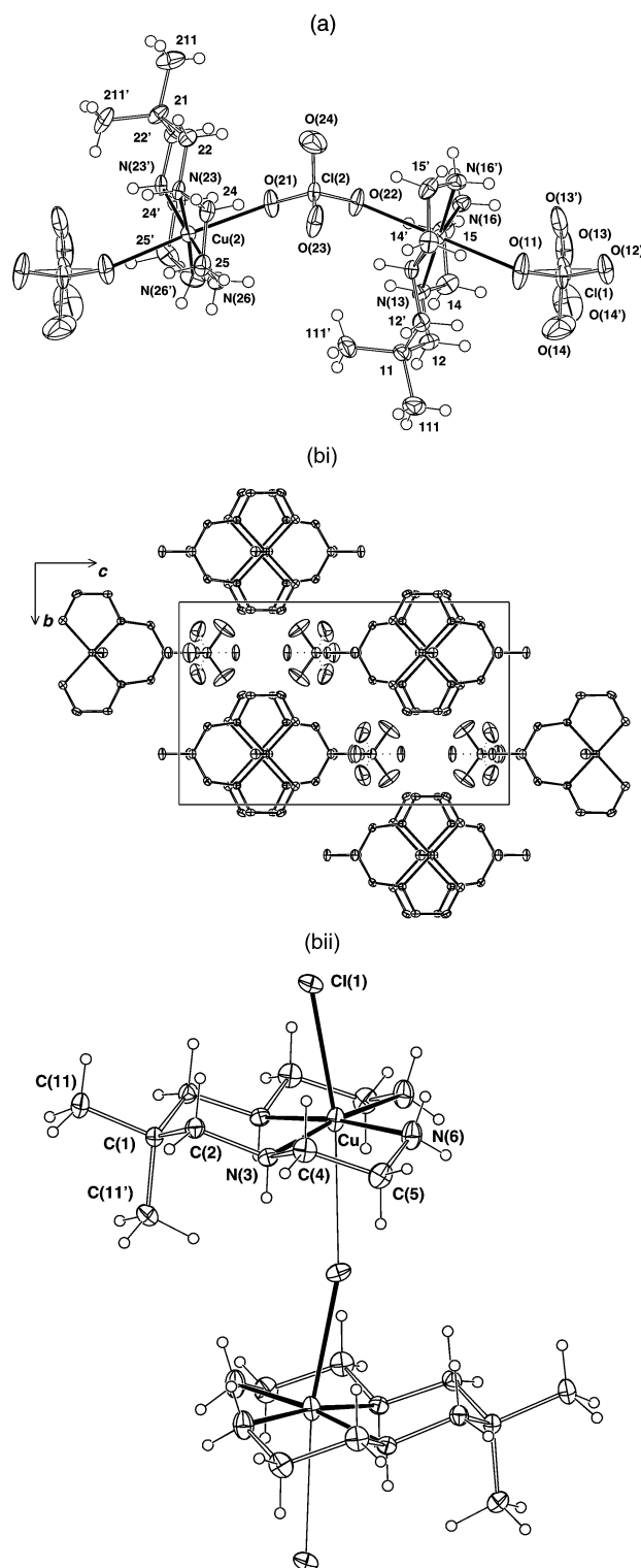
Fig. 5 (a) Section of the polymeric cation of [\text{CuL}^1(\text{OClO}_2\text{O})]_{(\infty)}\text{ClO}_4 , 1 ; a lies horizontal in the page. A figure showing the unit cell contents, projected down b , is deposited as ESI. (b) (i) The unit cell contents [\text{CuL}^1\text{Cl}]\text{ClO}_4 , 4 , projected down a , showing the columnar stacking of the cations and associated perchlorates up that axis. (ii) A side-on view of a cation stack, a lying vertically in the page.
